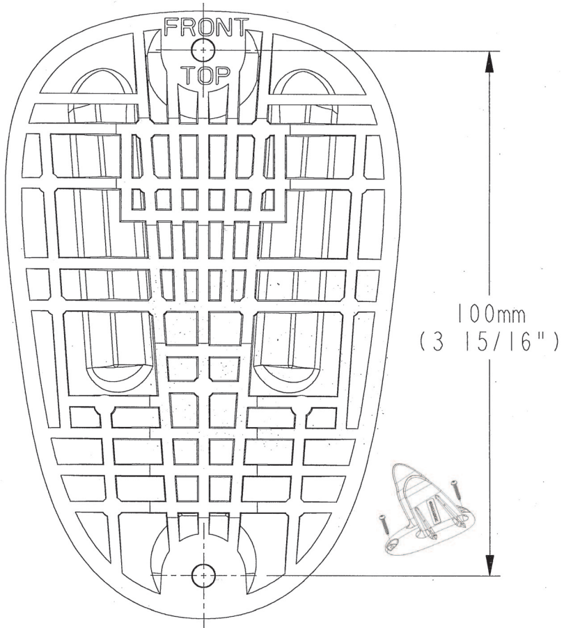
Figure 2. Drilling Template
